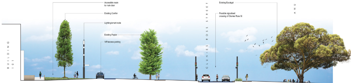
Section BB Scale 1:125
